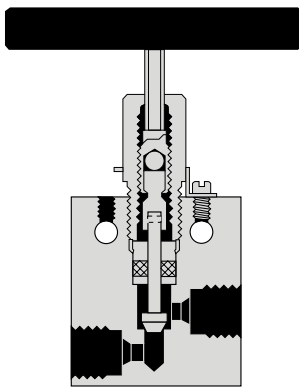
Pinned Stem
